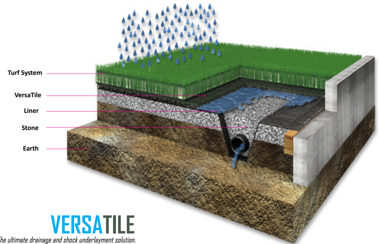
The design of the tile delivers 82% voids for unmatched vertical and horizontal drainage.
